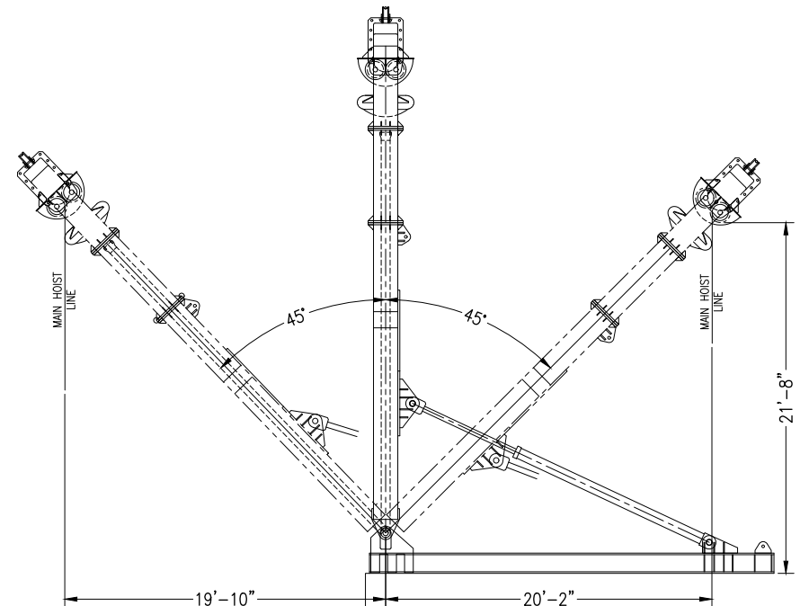
SIDE VIEW
